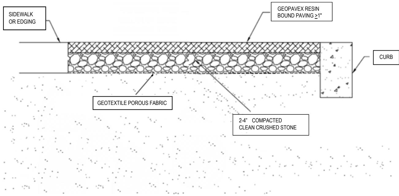
SECTION VIEW
