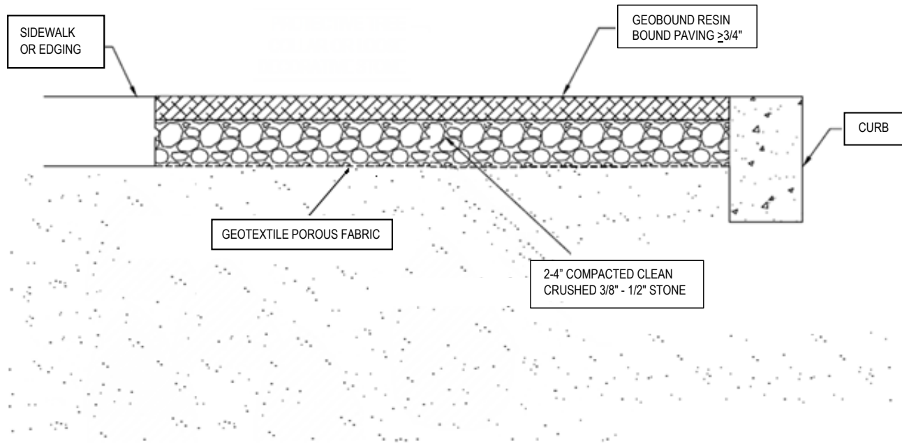
SECTION VIEW
