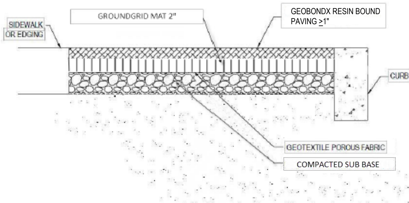
SECTION VIEW
