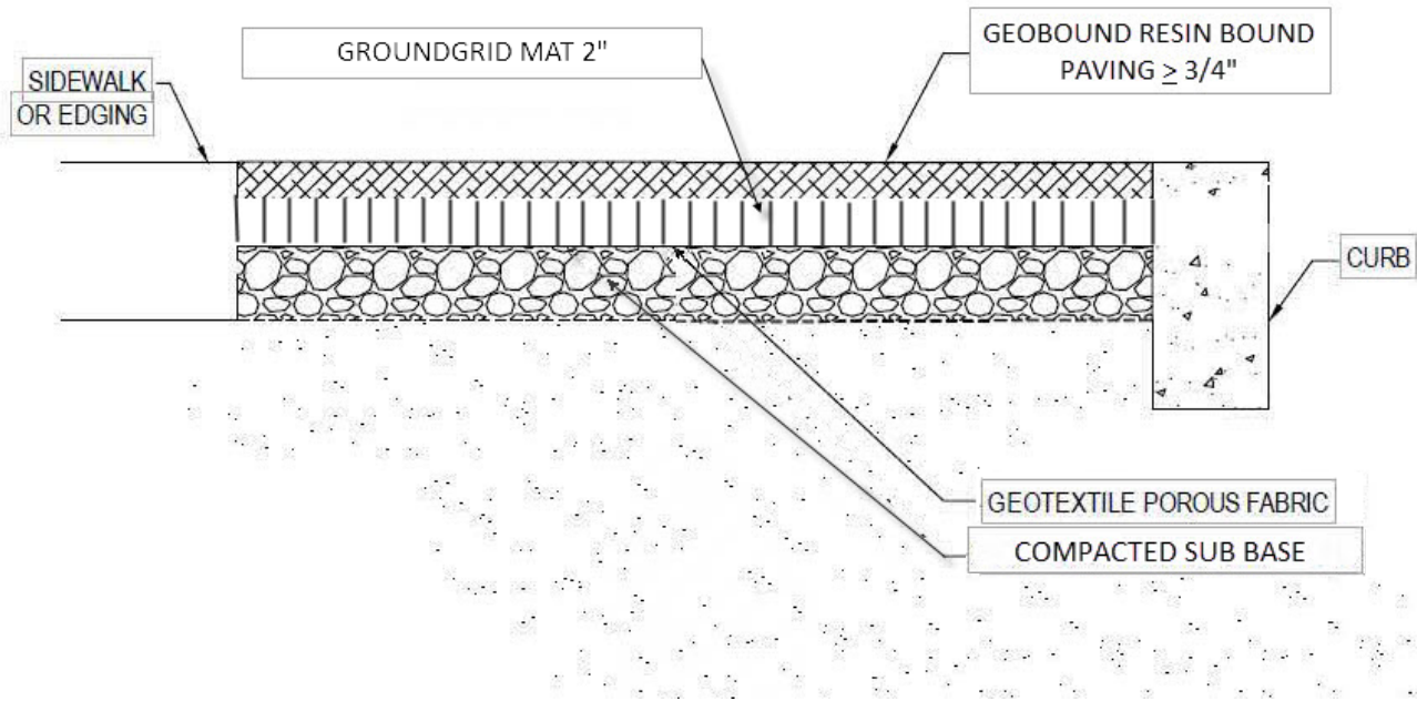
SECTION VIEW
